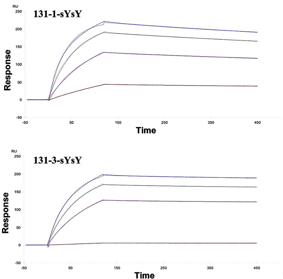
FIGURE 4: SPR sensorgrams (determined at 25 °C) for 131-1-sYsY and 131-3-sYsY showing binding to gp120. Colored lines represent sensorgram data, and overlaid black lines represent nonlinear fits.
