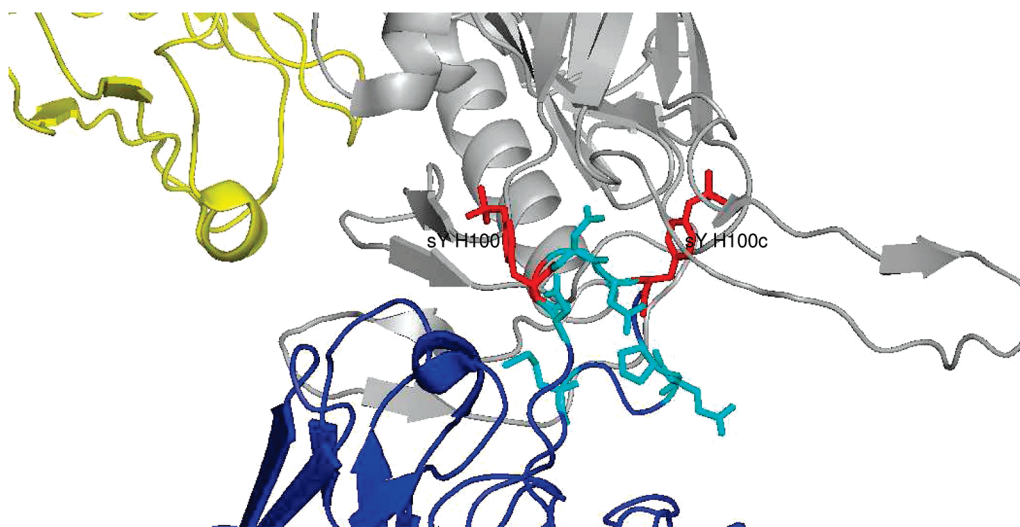
FIGURE 2: Sulfotyrosines (red) at the binding interface between 412d (blue) and gp120 (gray). Residues chosen for library randomization by site-saturation mutagenesis are colored cyan. CD4 is colored yellow. (Adapted from PDB: 2QAD).
