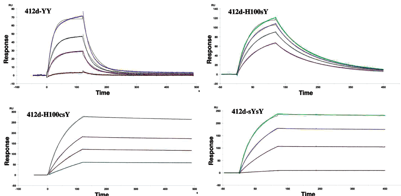
FIGURE 1: SPR sensorgrams (determined at 25 °C) for 412d-YY, 412d-H100sY, 412d-H100csY, and 412d-sYsY showing binding to gp120. Colored lines represent sensorgram data and overlaid black lines represent nonlinear fits.
