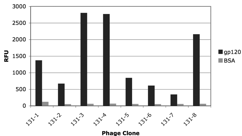
FIGURE 3: Binding of selected phage clones to gp120 and BSA based on ELISA analysis (only single measurements were taken). For each sample, 3.2 \times 10^7 phage particles were loaded.
